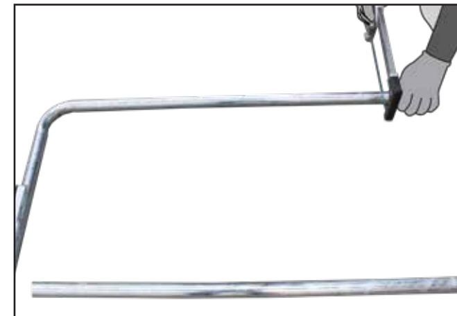
I. Using a hacksaw or similar, carefully cut through the top, bottom tubes, the toeboard and the mid rail as shown. For galvanised assemblies, spray with Galvafroid or similar to prevent corrosion.
